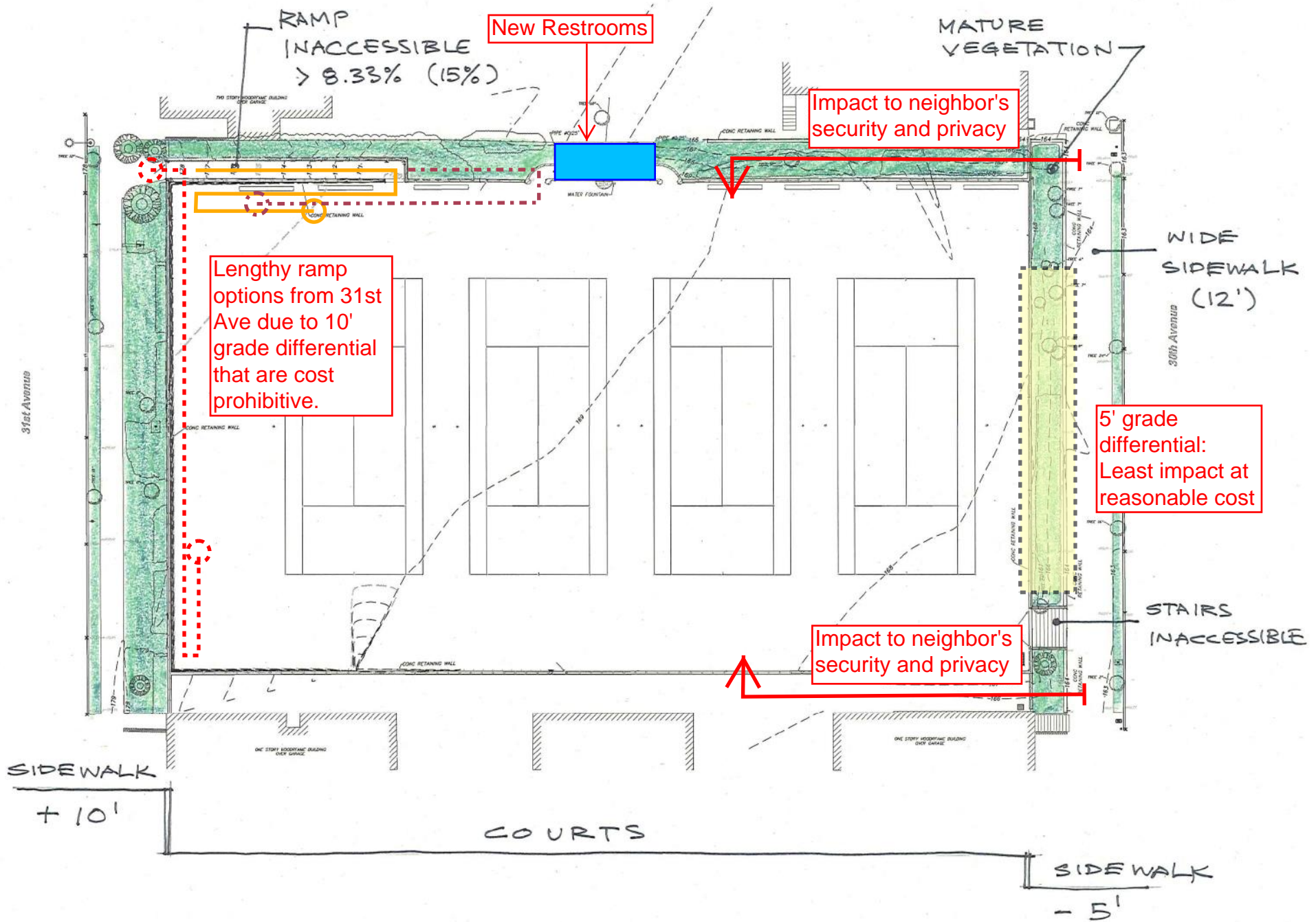
WHEELCHAIR-ACCESSIBLE RAMP STUDIES
